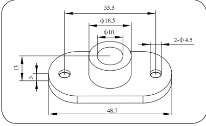
20-120 Köşe Kiliti/Corner Lock
