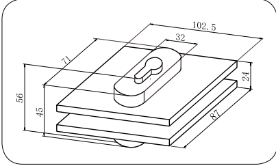
20-120 Köşe Kiliti/Corner Lock
