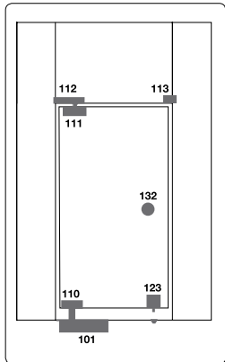
Cam Detaylı Set 1 Glass Detailed Set 1
